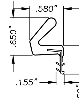
16 WEATHERSTRIPPING QEBD-650 FOAM
