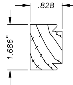
12 LATCH STILE WOOD REINFORCEMENT
