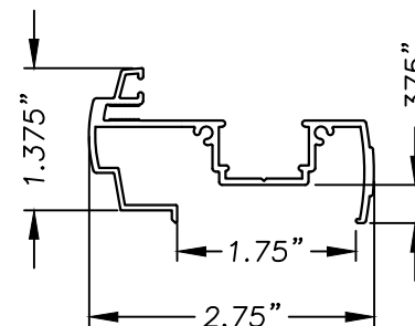
② HINGE STILE WOOD REINFORCEMENT
