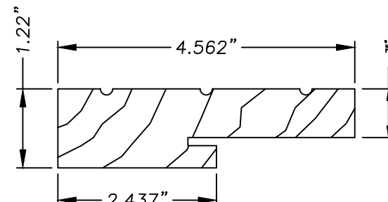
② HINGE STILE WOOD REINFORCEMENT
